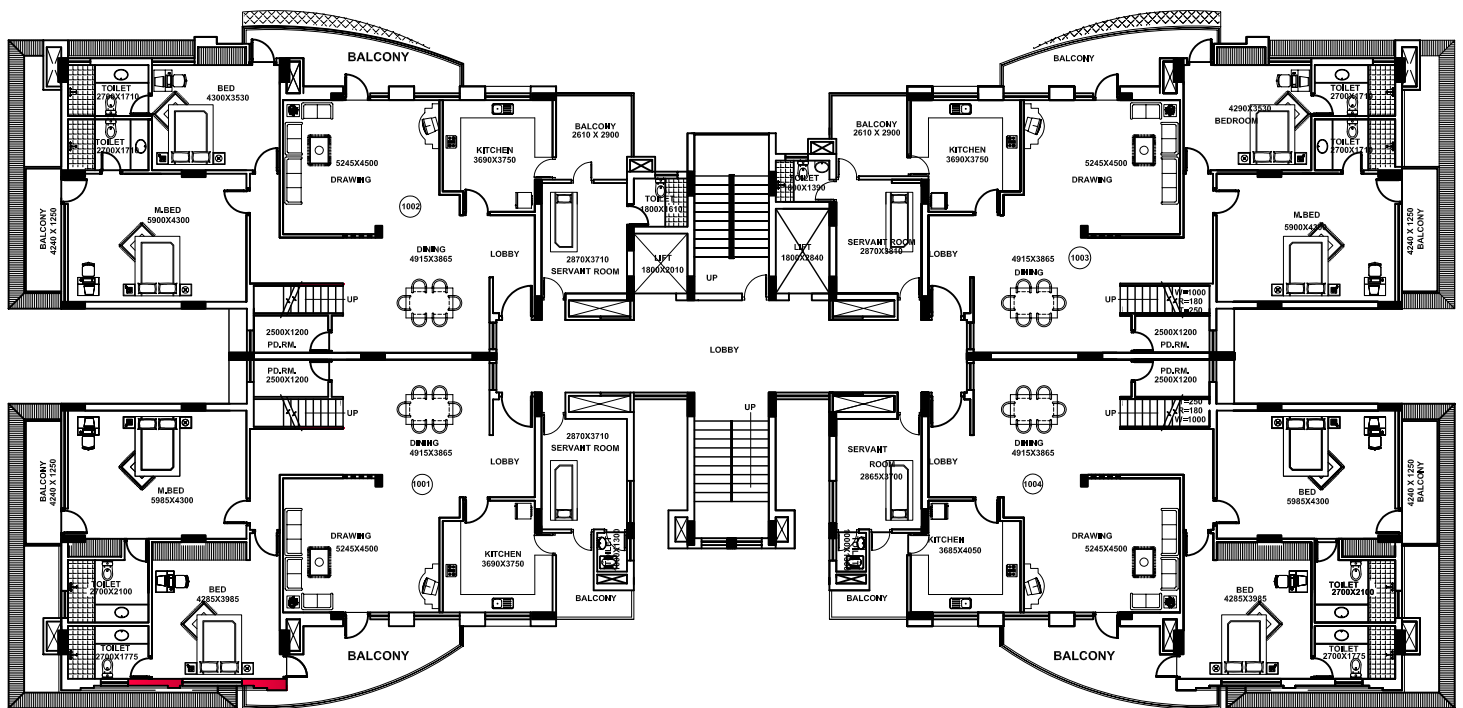
TENTH FLOOR PLAN (PENT HOUSE LEVEL.- I)
